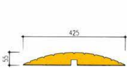
SECTION
